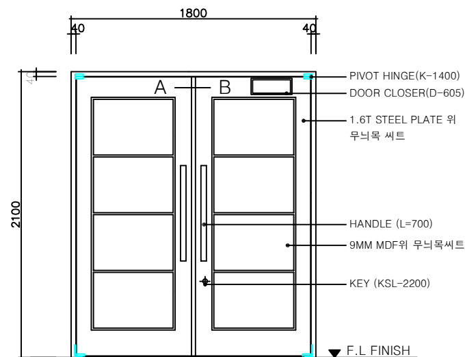
DOUBLE DOOR (SCALE 1/NONE)
