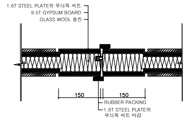
A - B SECTION (SCALE 1/5)
