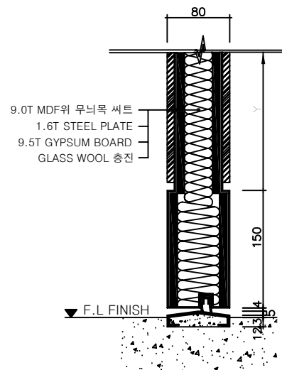
SILL SECTION (SCALE 1/5)
