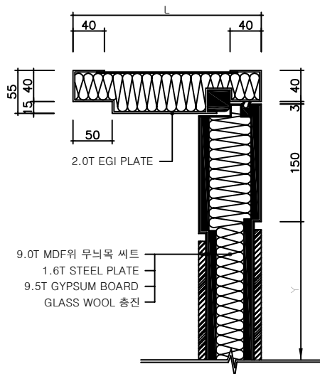
HEAD SECTION (SCALE 1/5)
