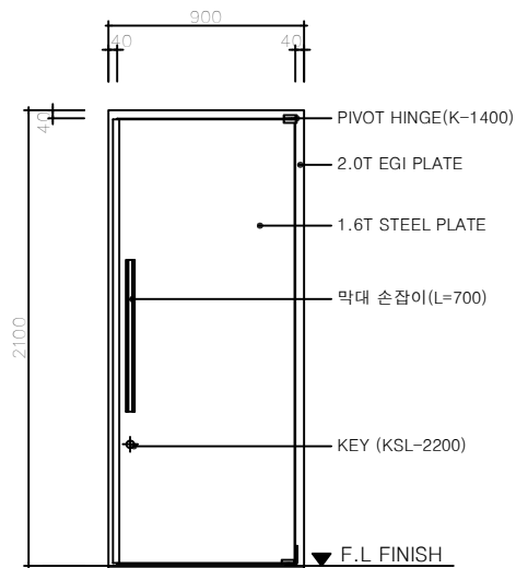
SINGLE DOOR (SCALE 1/NONE)
