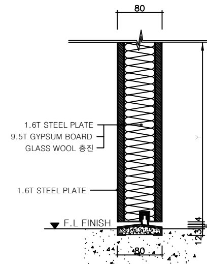
SILL SECTION (SCALE 1/5)
