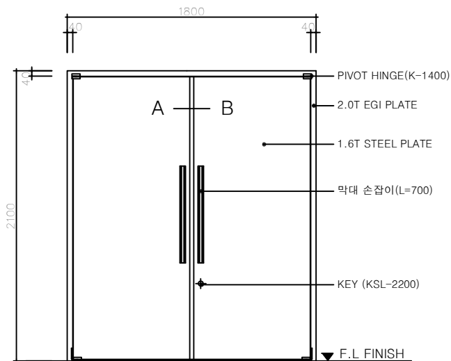
DOUBLE DOOR (SCALE 1/NONE)
