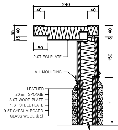
HEAD SECTION (SCALE 1/5)
