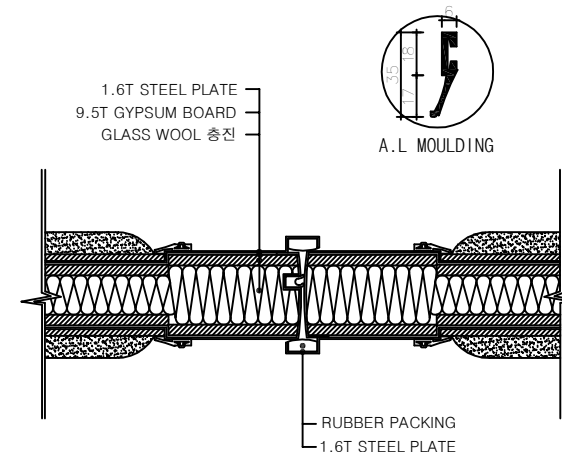
A - B SECTION (SCALE 1/5)
