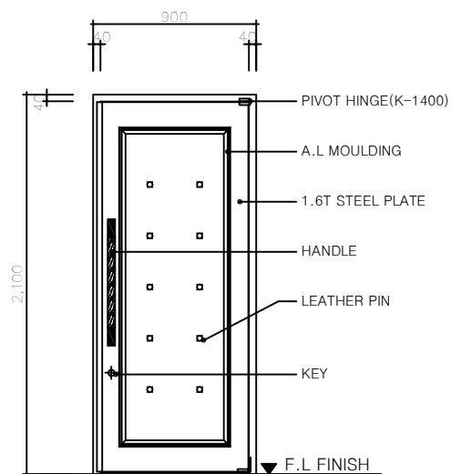
SINGLE DOOR (SCALE 1/NONE)
