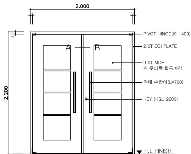
DOUBLE DOOR (SCALE 1/NONE)
