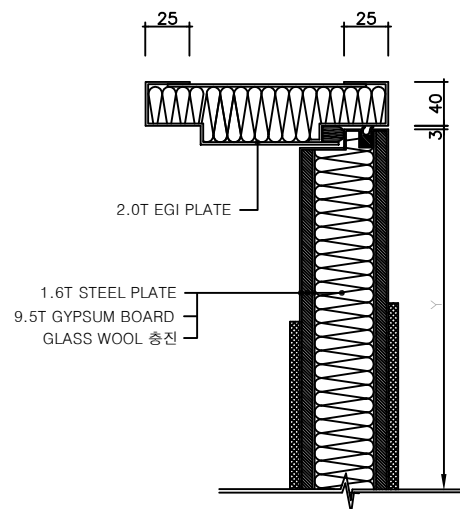
HEAD SECTION (SCALE 1/5)
